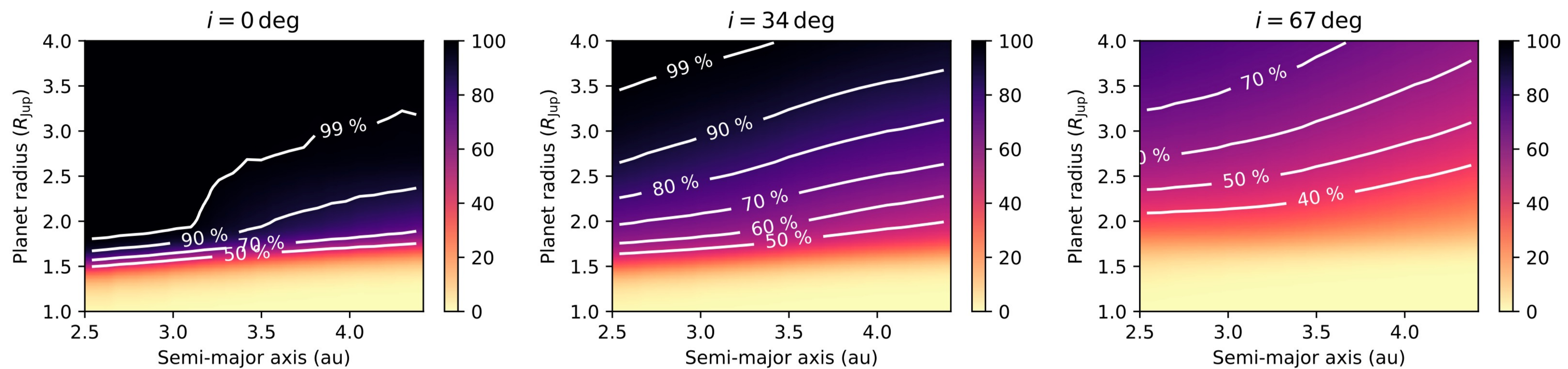
Fig. 1 Detectability of planets around epsi Eridani for which a planet of given radius would have been detected by K-Stacker, for 3 different values of the inclination. The inclination has a significant impact on the detectability of planets, due to the influence of the phase angle on the polarization contrast.
